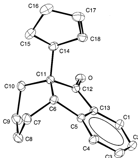
Figure 1. Molecular structure of 12 as found by X-ray crystallography; hydrogen atoms are omitted for clarity; thermal ellipsoids are drawn at the 50% probability level
